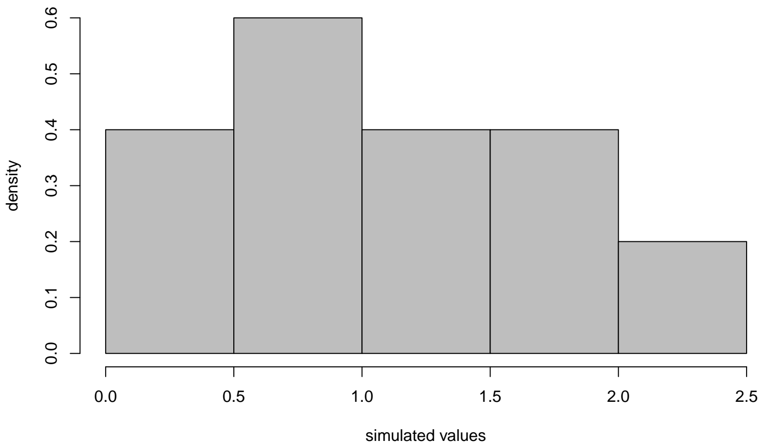
Histogram of 1st simulated series
