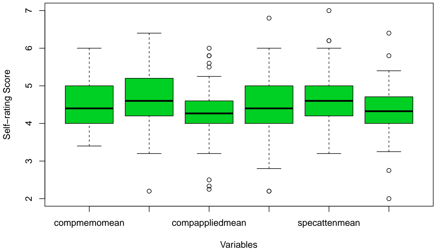
Memo/Attention/Applied Mean
