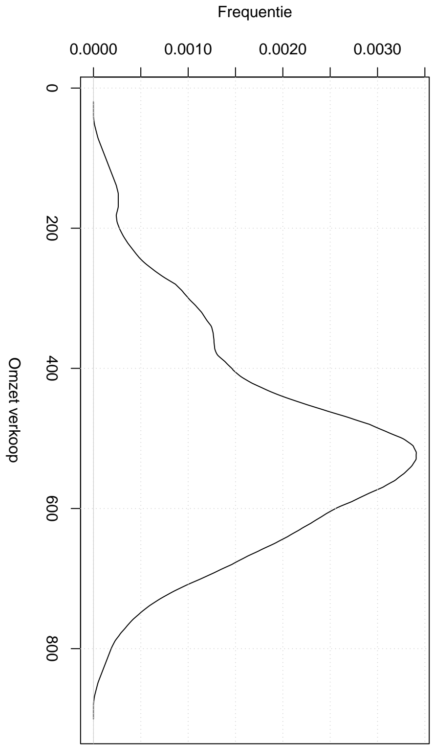
Triangular Kernel
