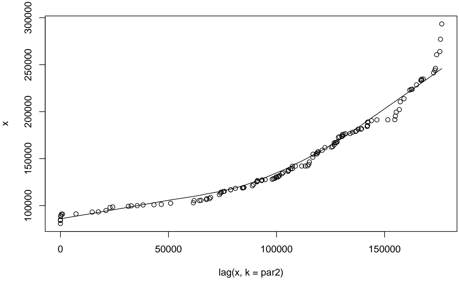
Lag plot (k=36), and lowess
