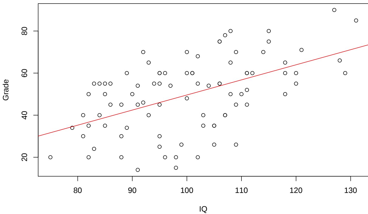
Regression Solution
