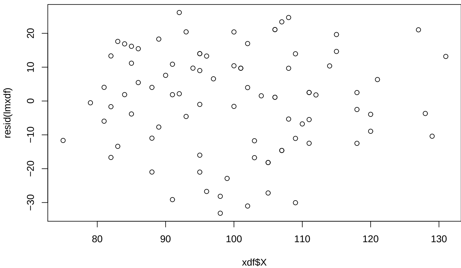
Scatterplot of Residuals of Model Fit
