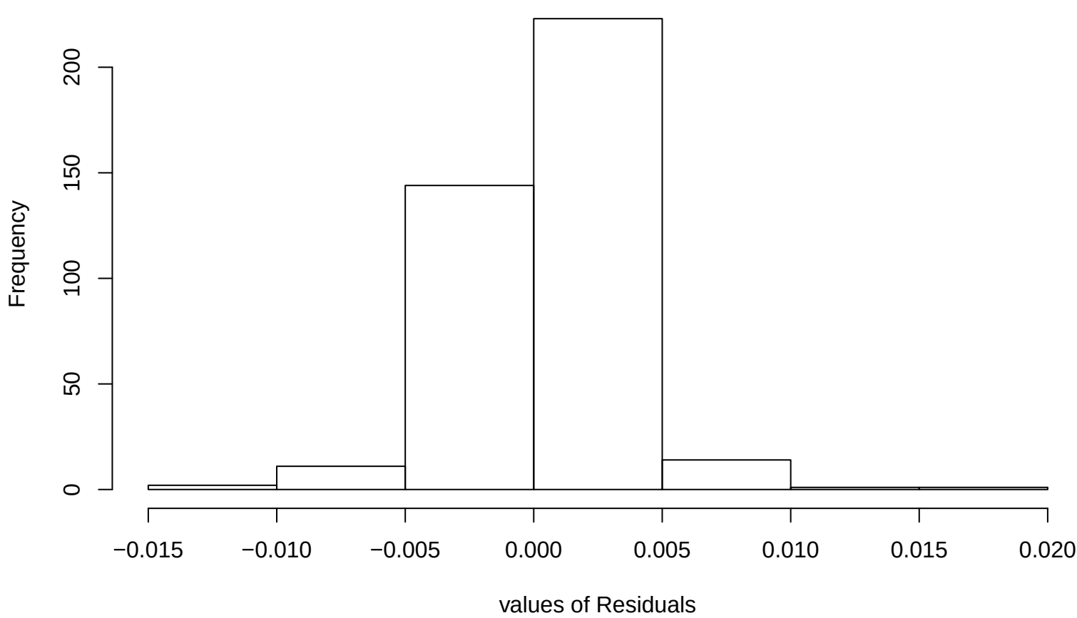
Residual Histogram
