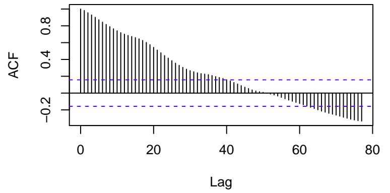
Standardized Residuals
