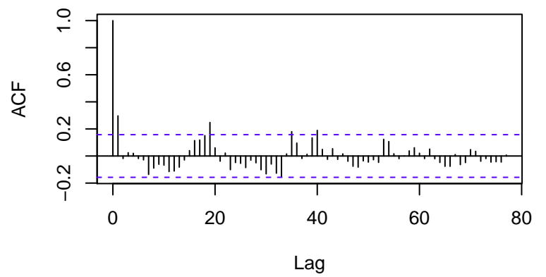
Standardized Residuals
