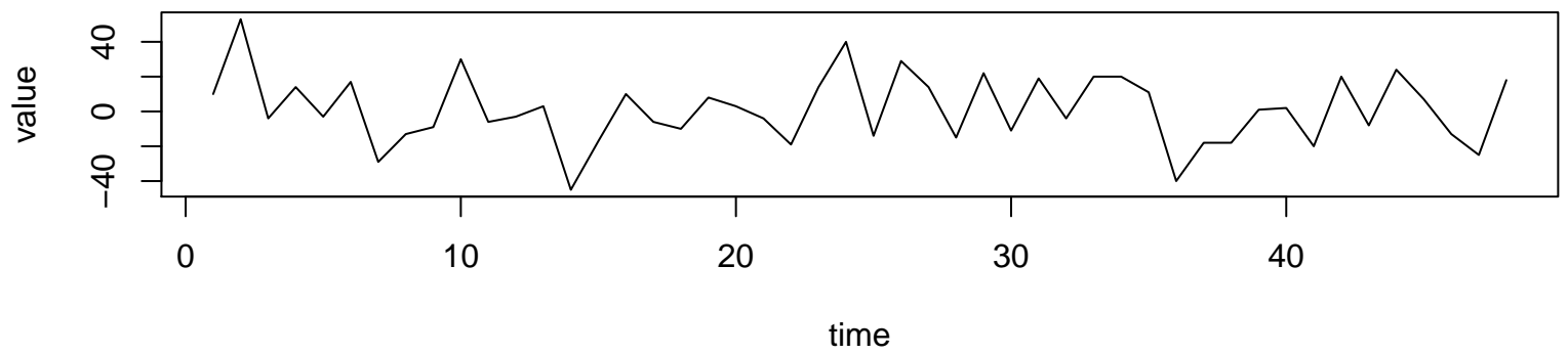
Working Time Series ( \lambda=1, d=0, D=2 )
