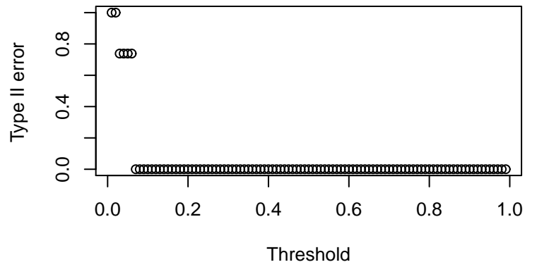
1 - Sensitivity
