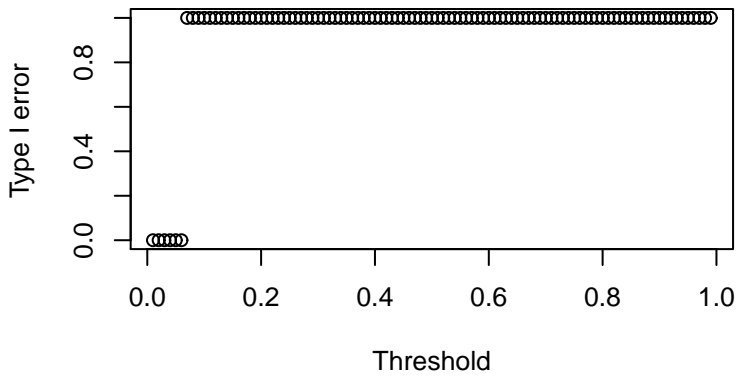
1 - Specificity
