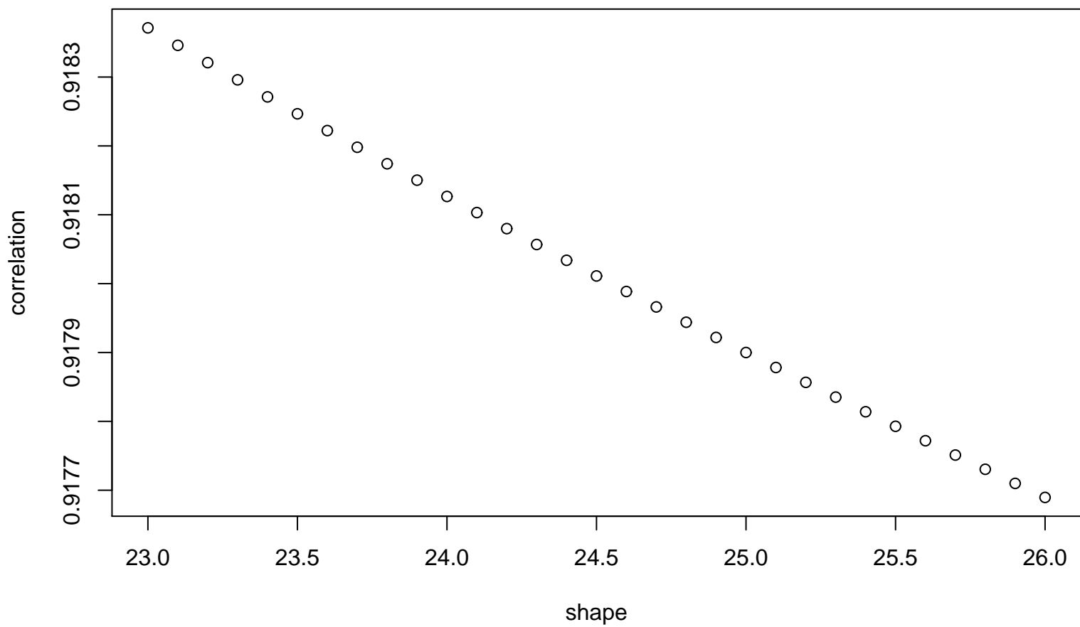
PPCC Plot – Weibull
