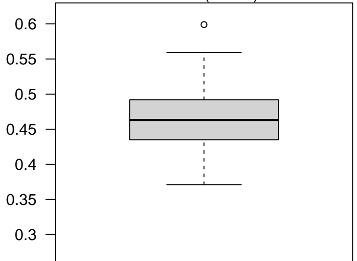
Node 3 (n = 38)
