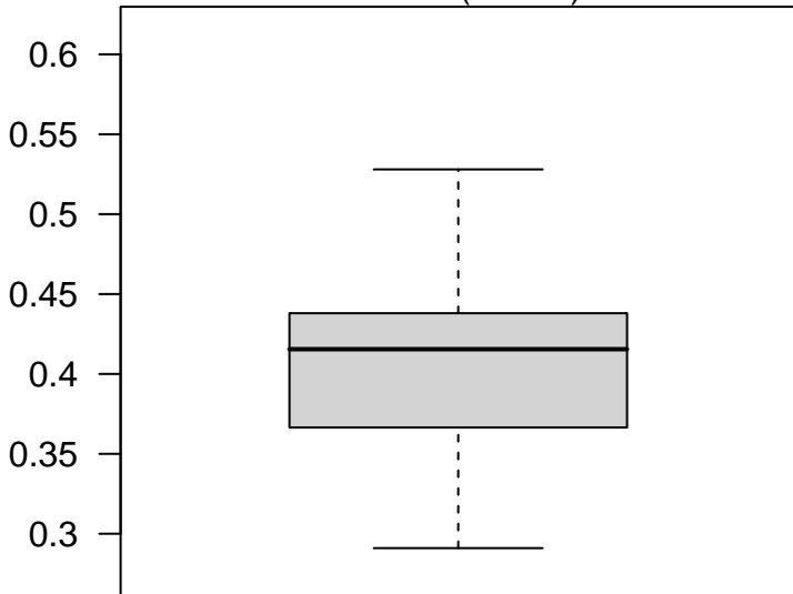
Node 2 (n = 16)
