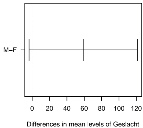
95% family-wise confidence level
