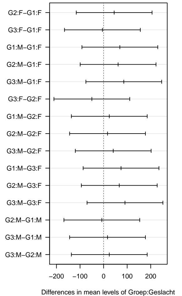
95% family-wise confidence level
