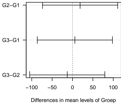
95% family-wise confidence level
