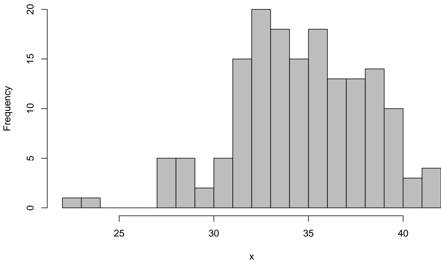
Histogram separate-score
