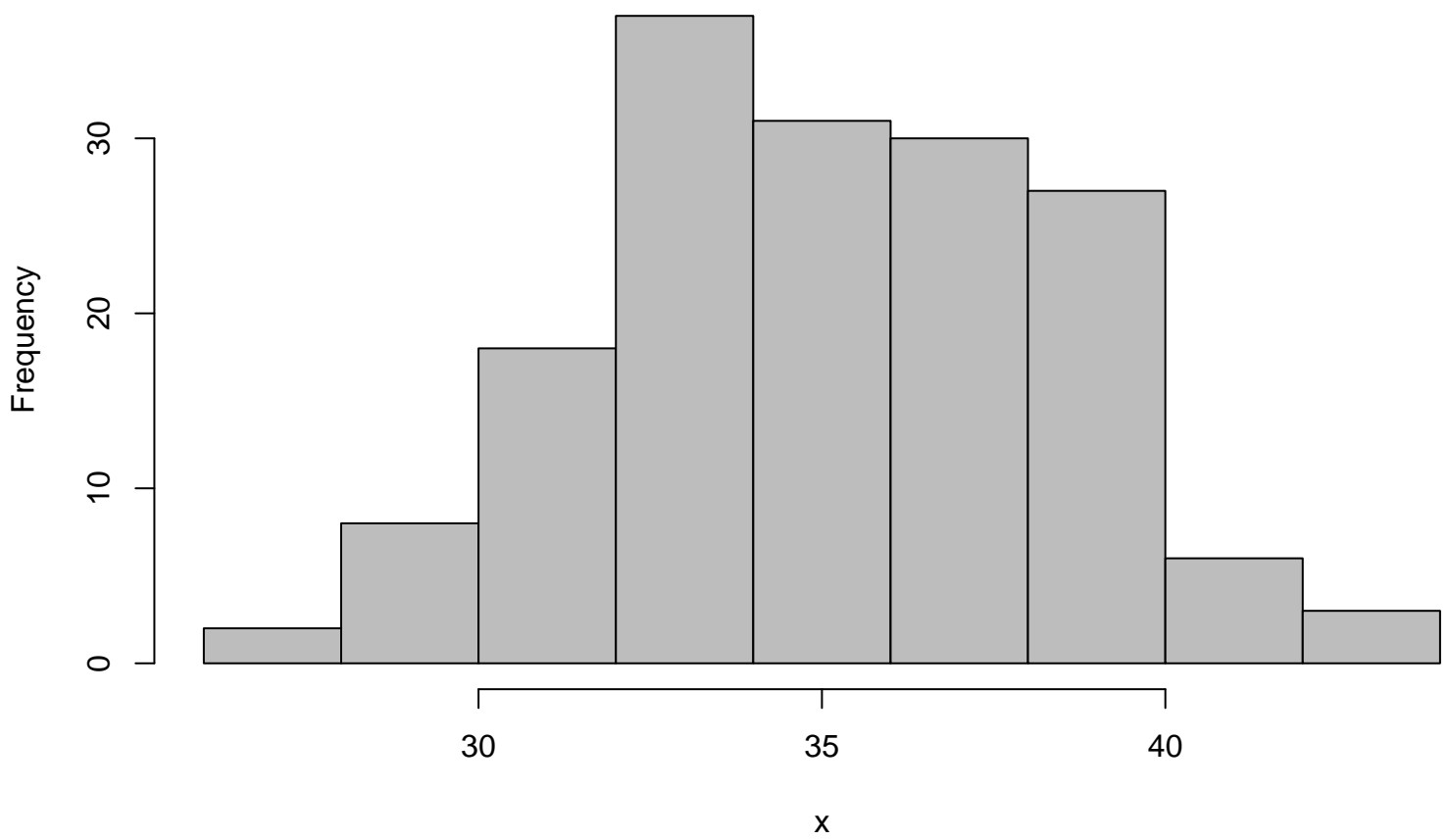
Histogram Connected-score
