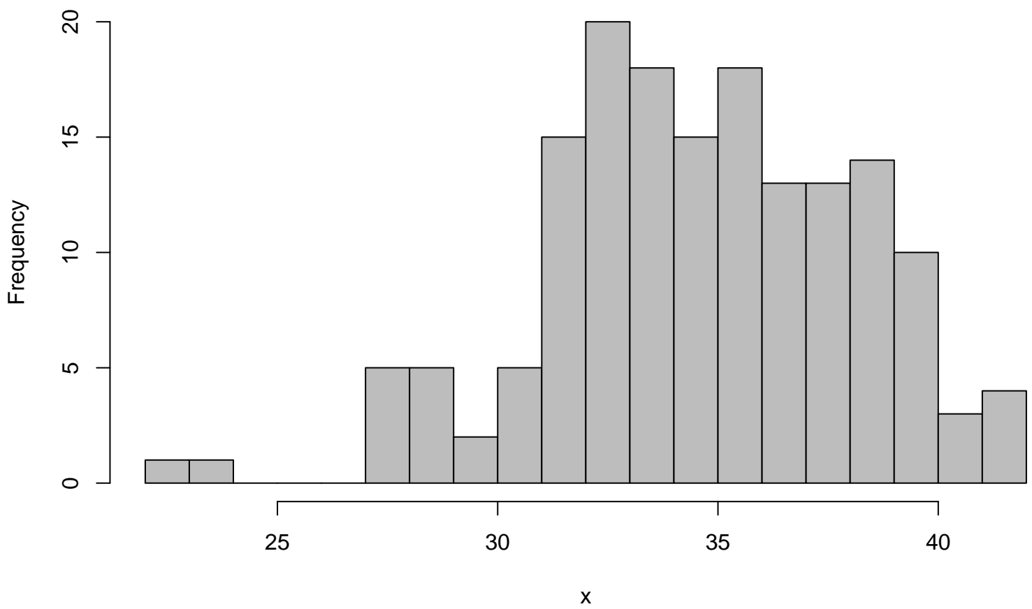
Histogram Seperate-score
