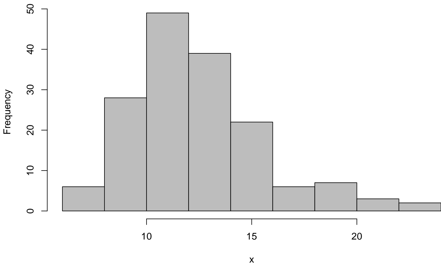
Histogram: Depression
