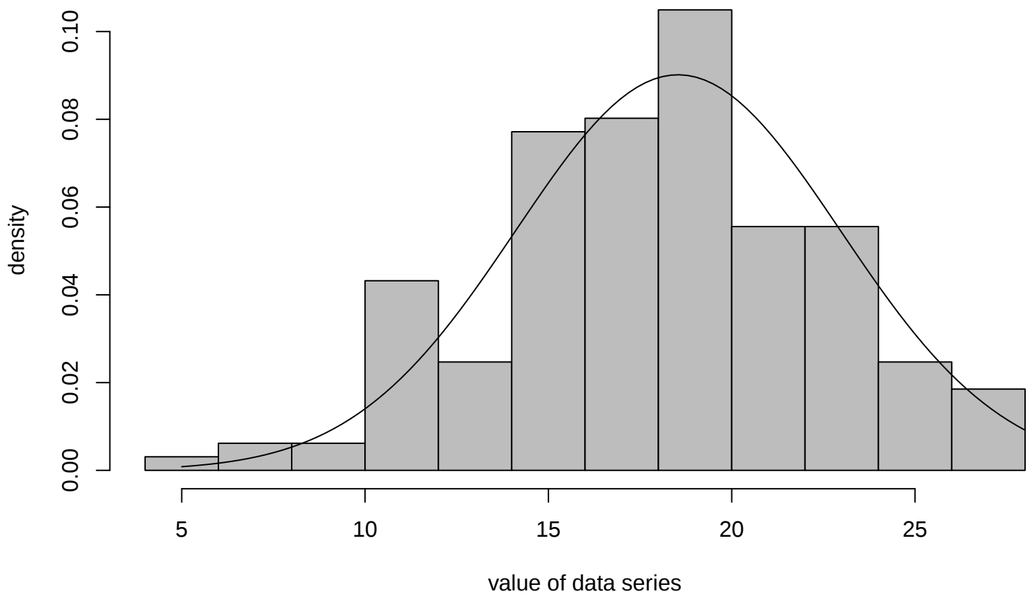
Histogram and Fitted Normal Density
