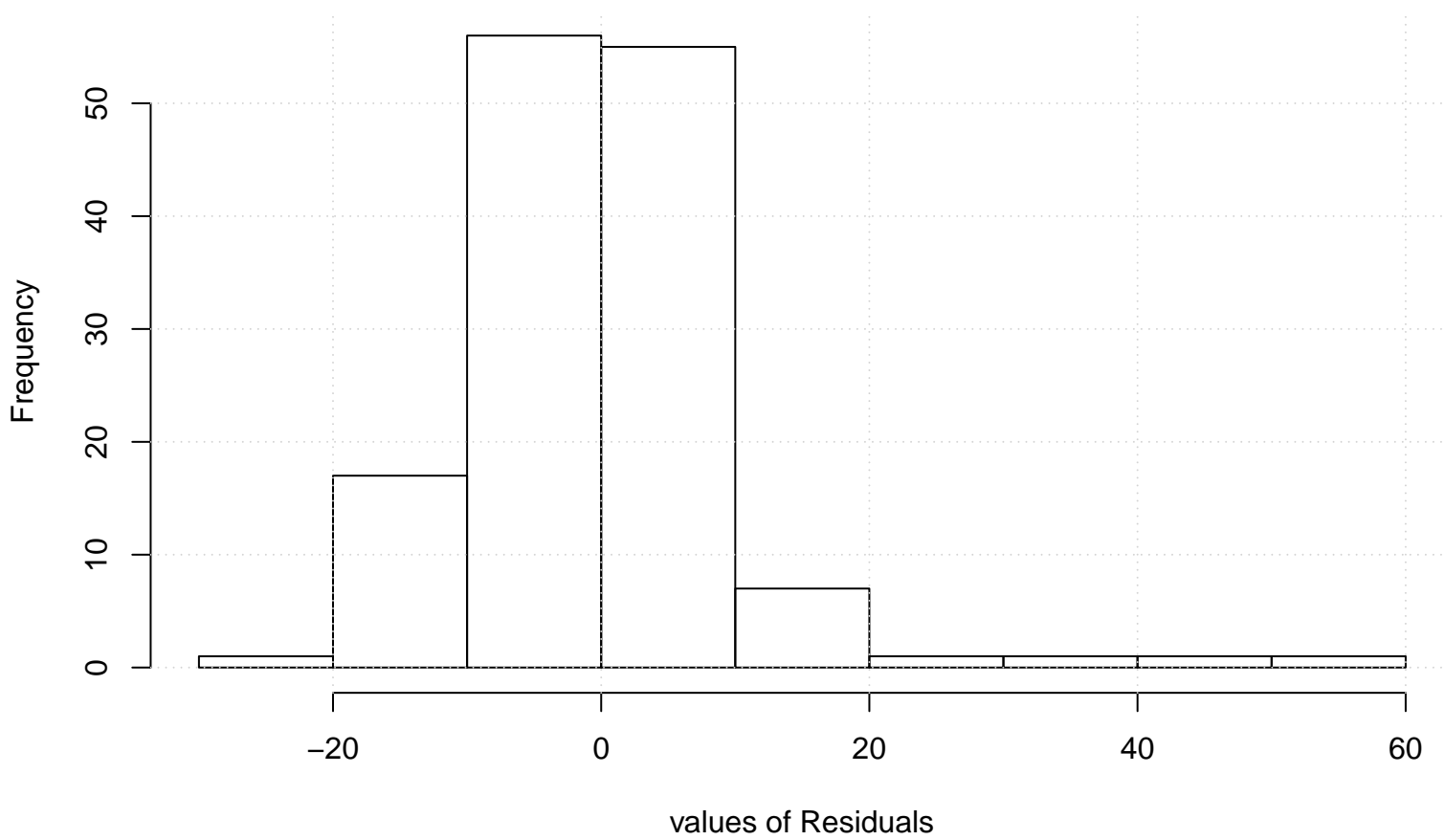
Residual Histogram
