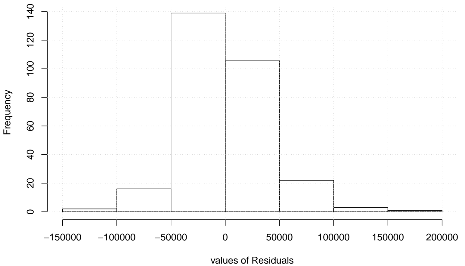
Residual Histogram
