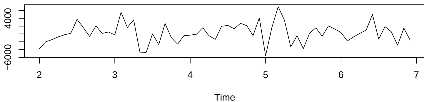
Interpolation Prediction Errors
