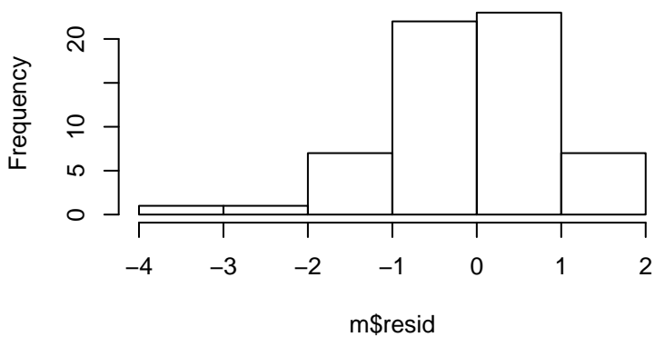
Residual Histogram
