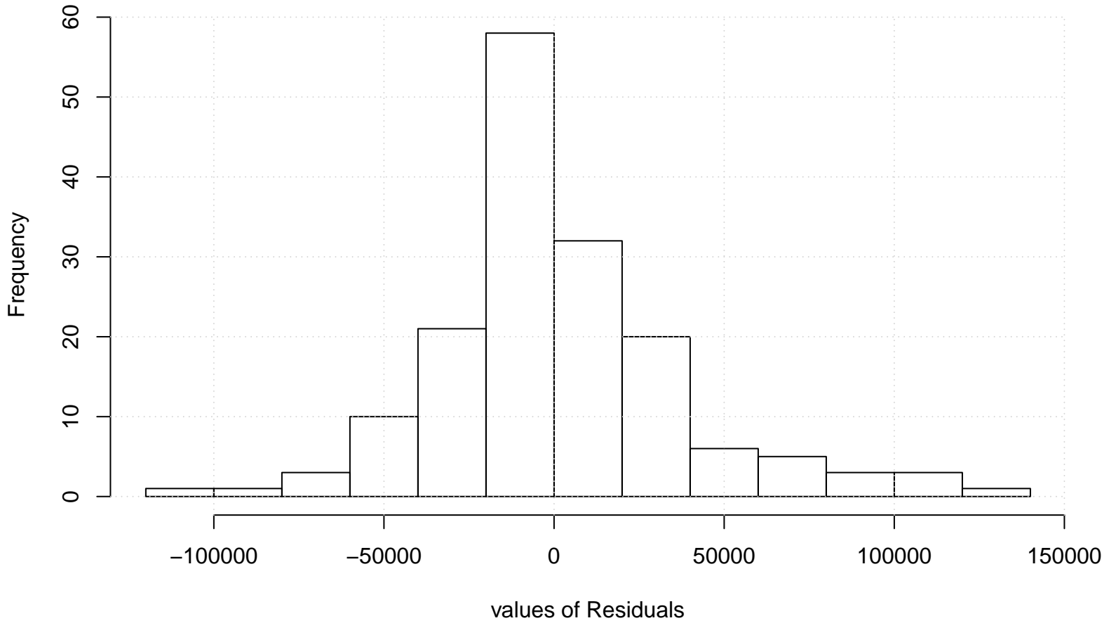
Residual Histogram
