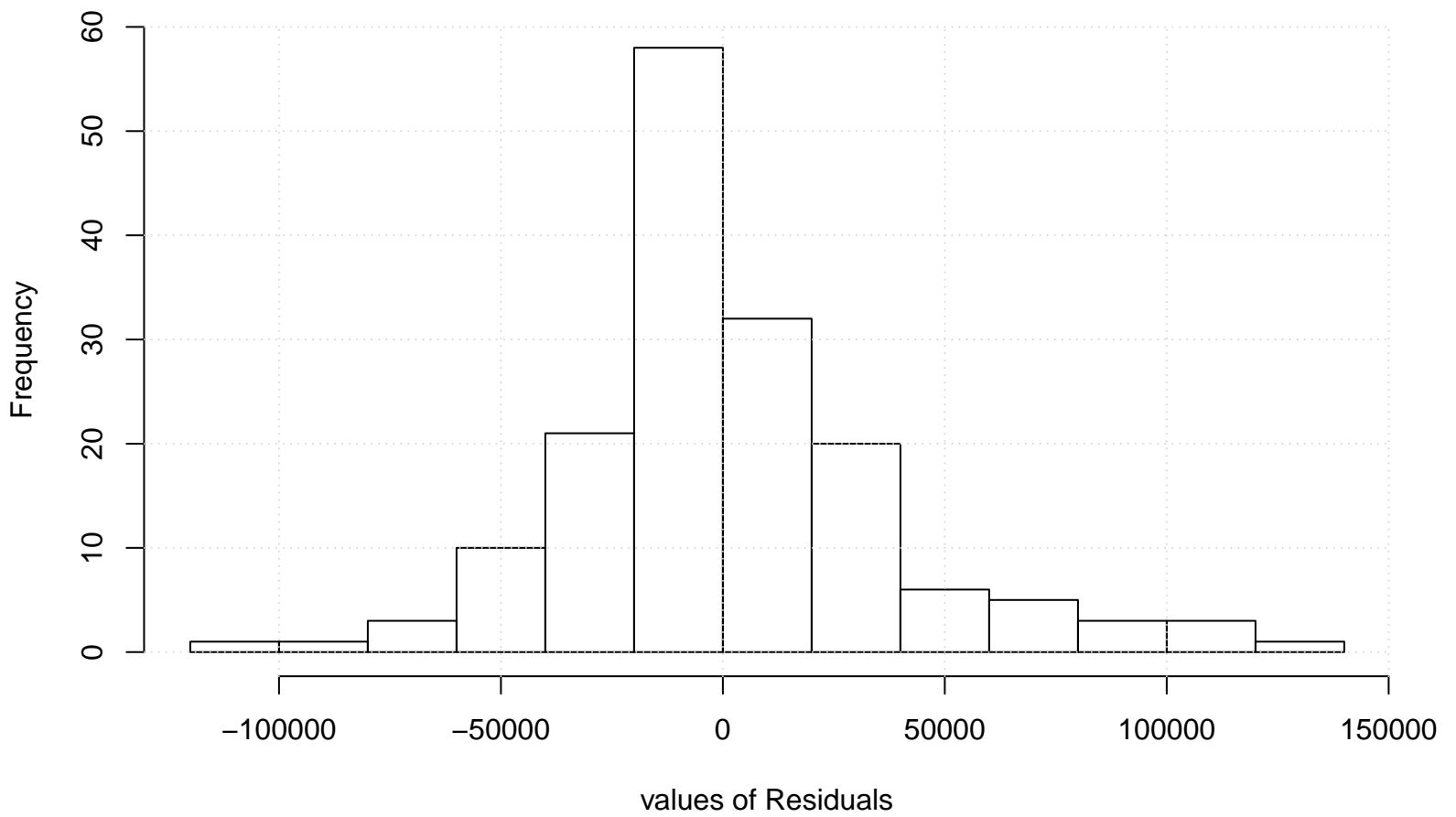
Residual Histogram
