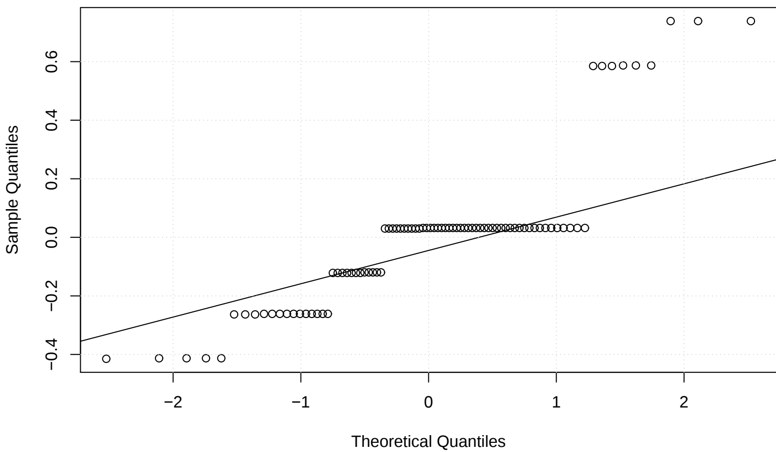
Residual Normal Q-Q Plot
