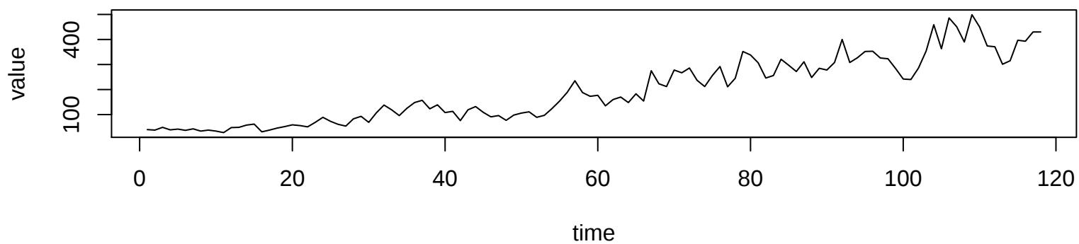
Working Time Series ( \lambda=1 , d=0 , D=0 )
