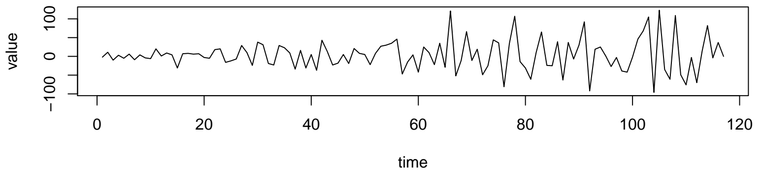
Working Time Series ( \lambda=1 , d=1 , D=0 )
