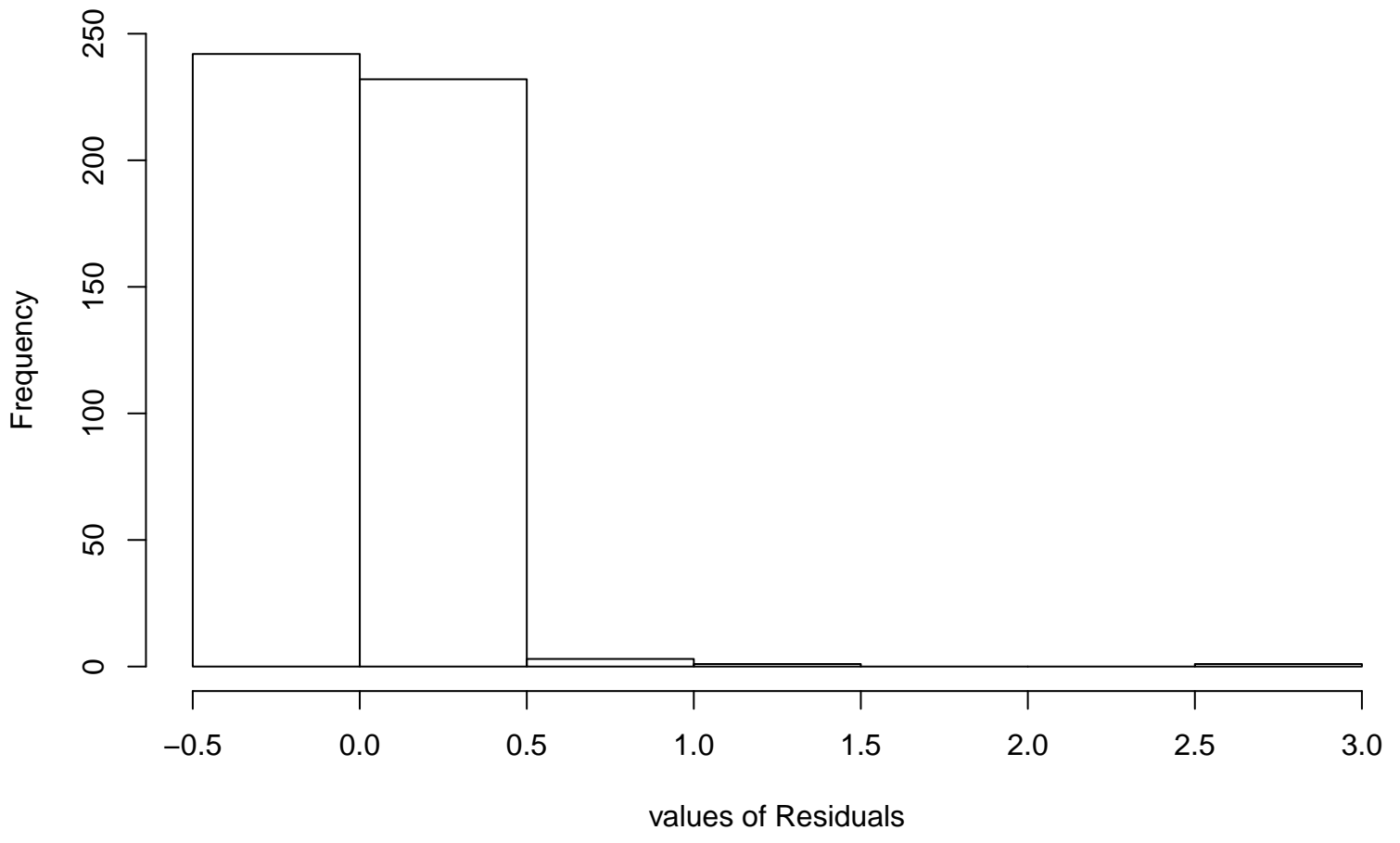
Residual Histogram
