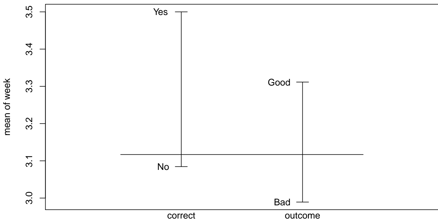
Design Plot of Group Means
