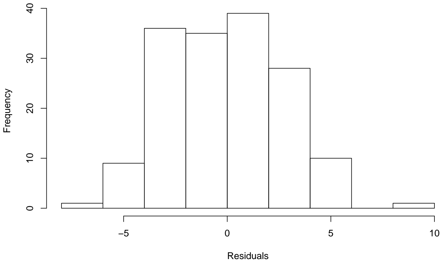
Residual Histogram
