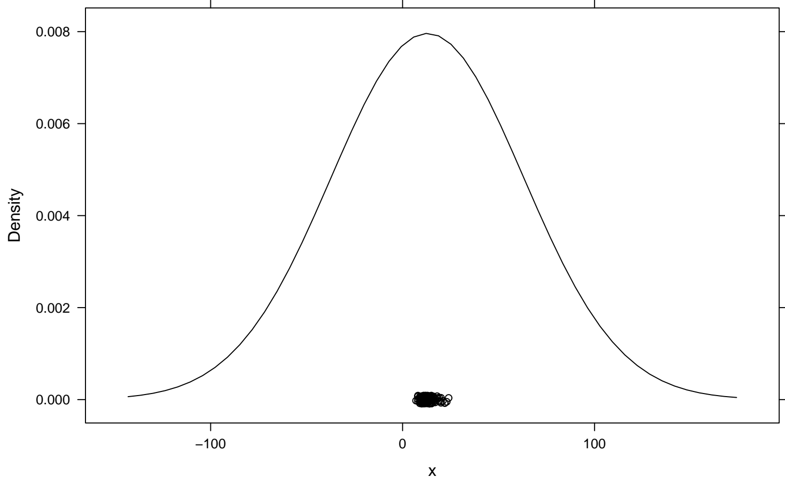
Density Plot bw = 50
