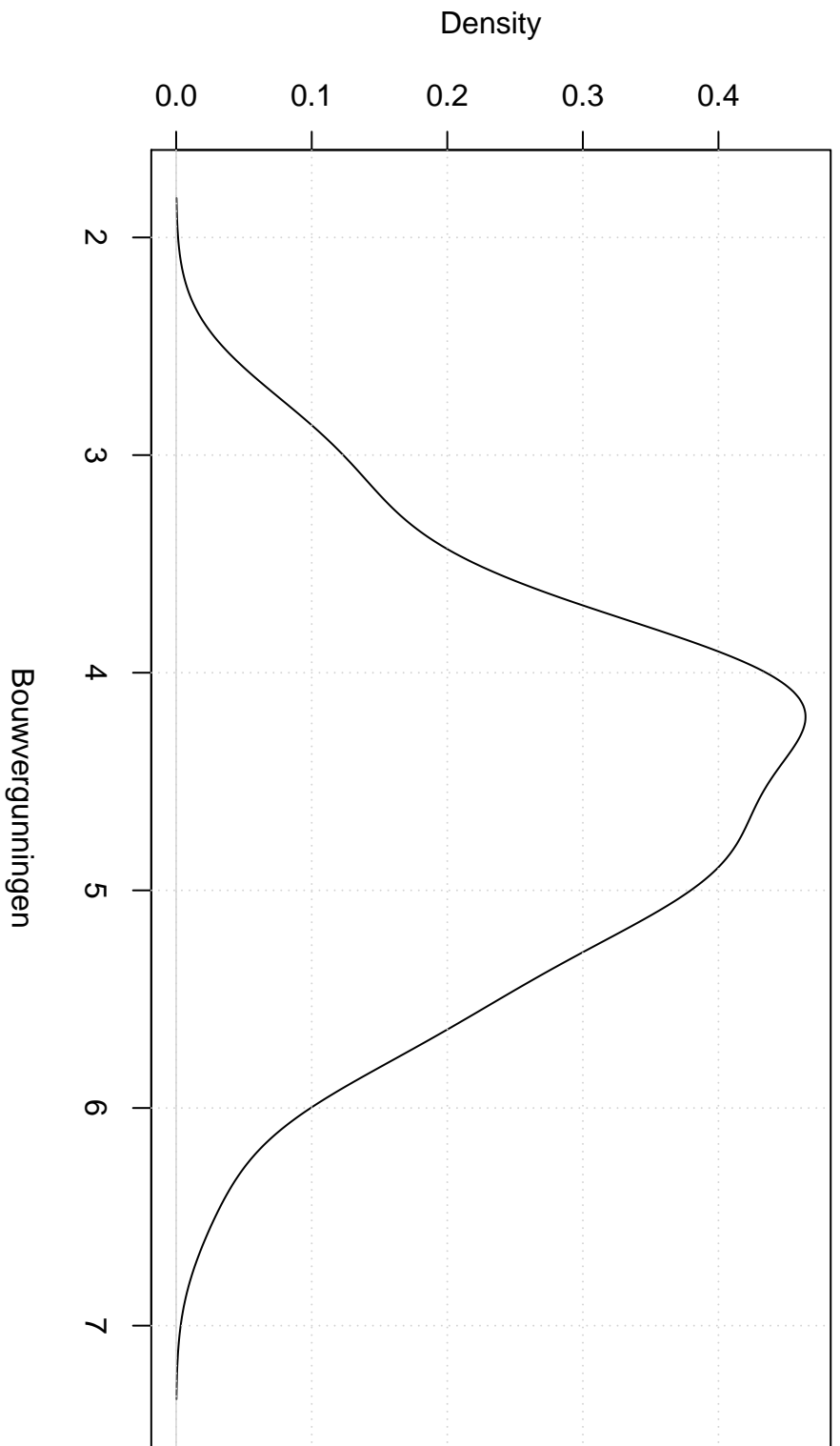
Gaussian Kernel
