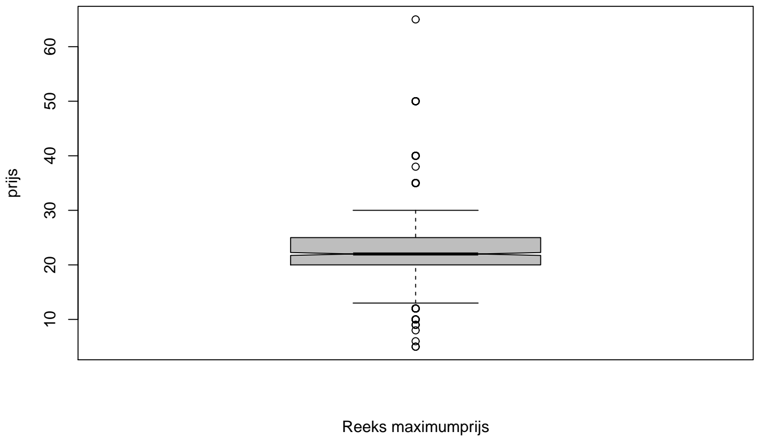
Boxplot maximumprijs
