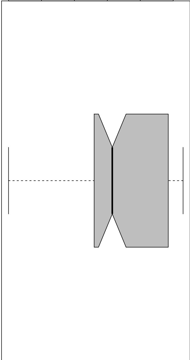
Notched Boxplots
