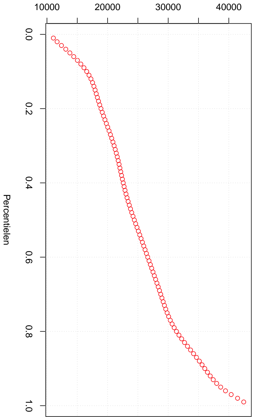
Harrell-Davis Quantiles
