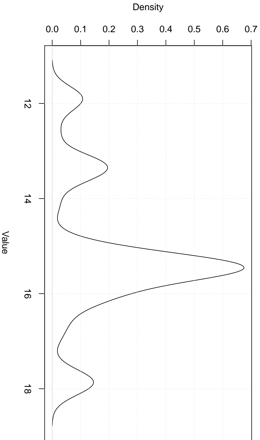
Gaussian Kernel
