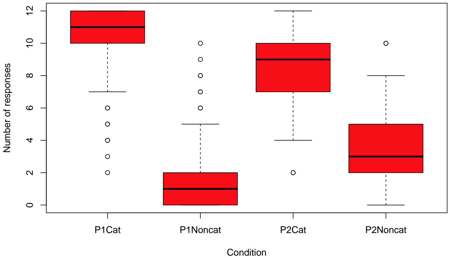
Box plot for the distribution of scores
