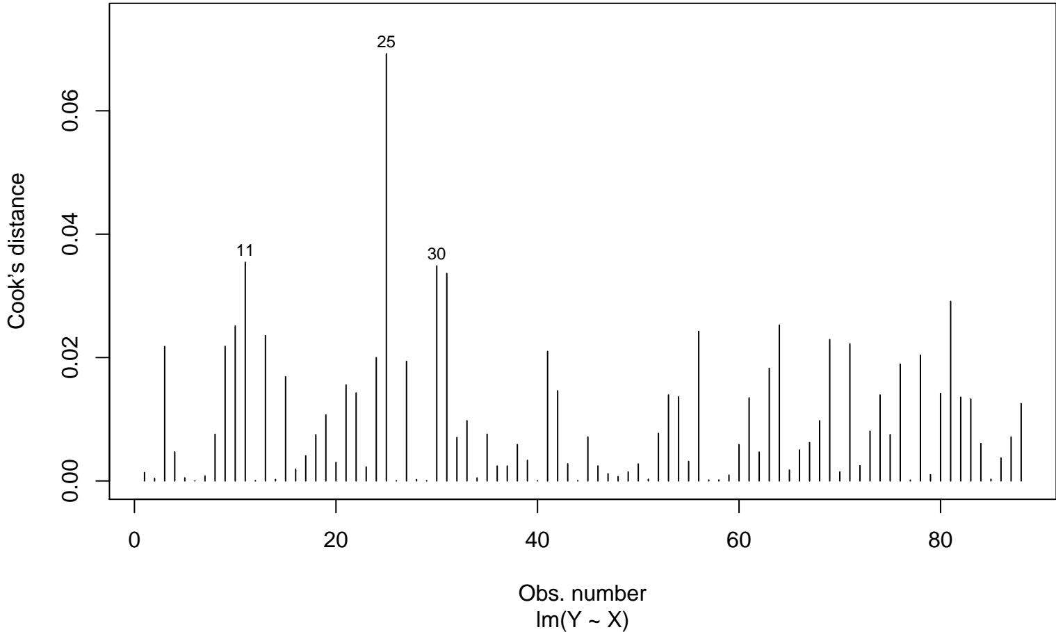
Cook's distance
