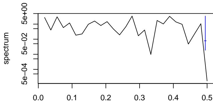
Standardized Residuals
