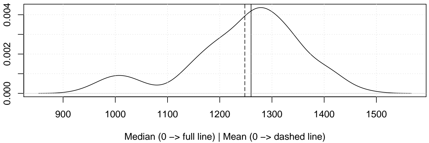
Density Plot – Gaussian Kernel
