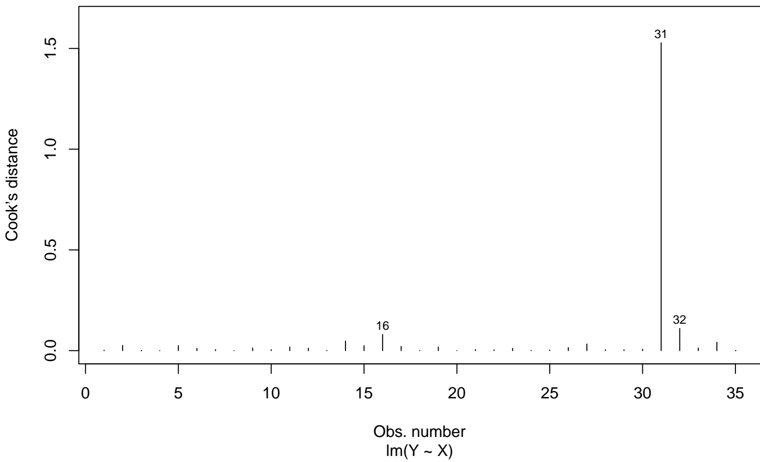
Cook's distance
