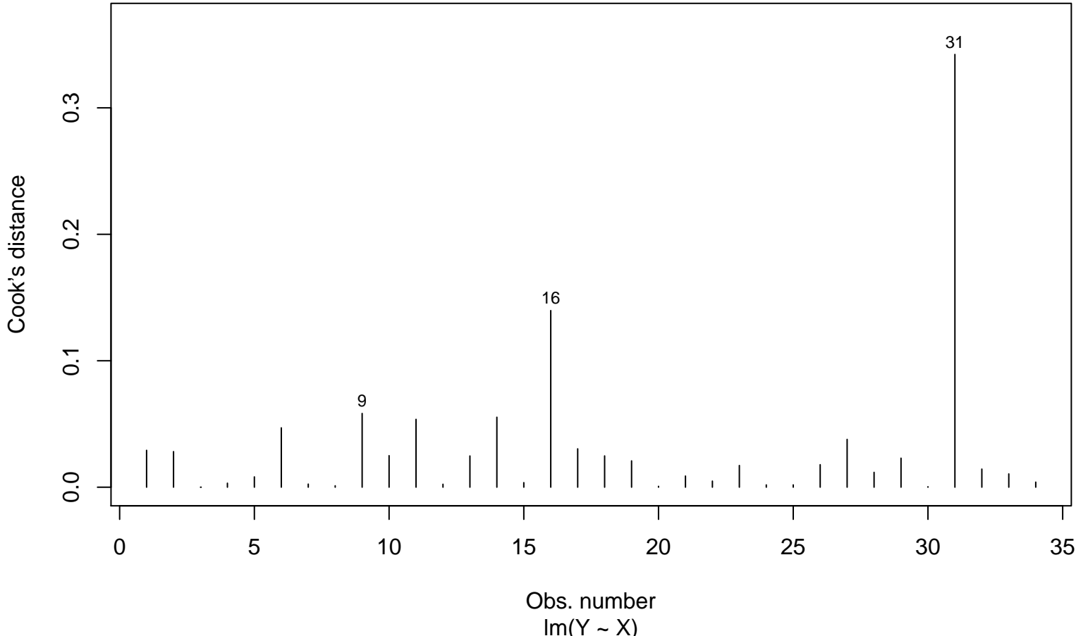
Cook's distance
