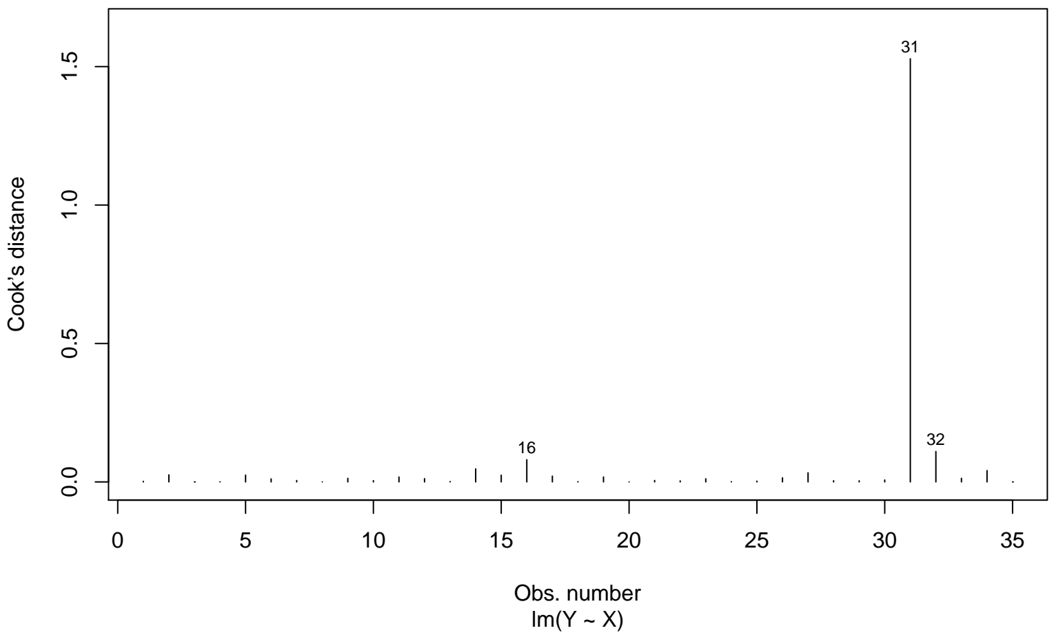
Cook's distance
