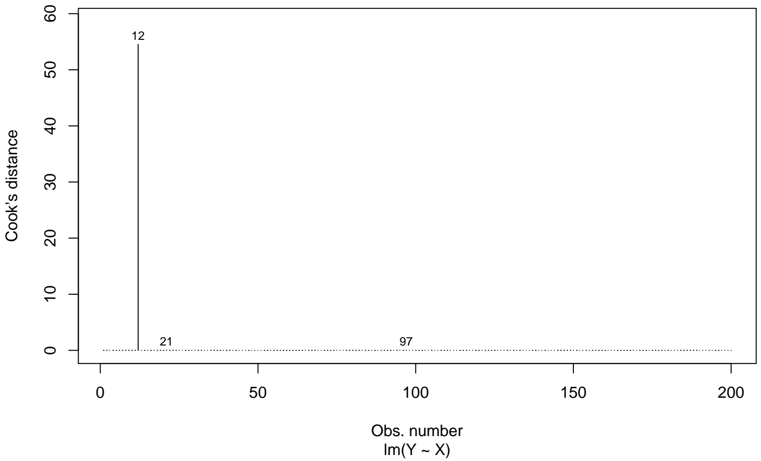
Cook's distance
