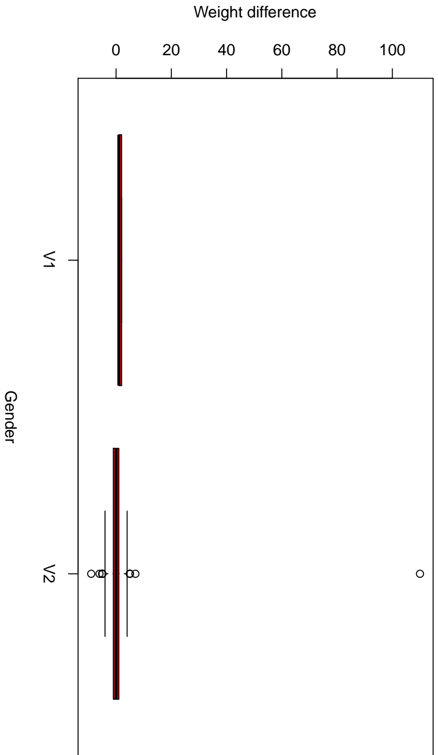
Boxplots Title
