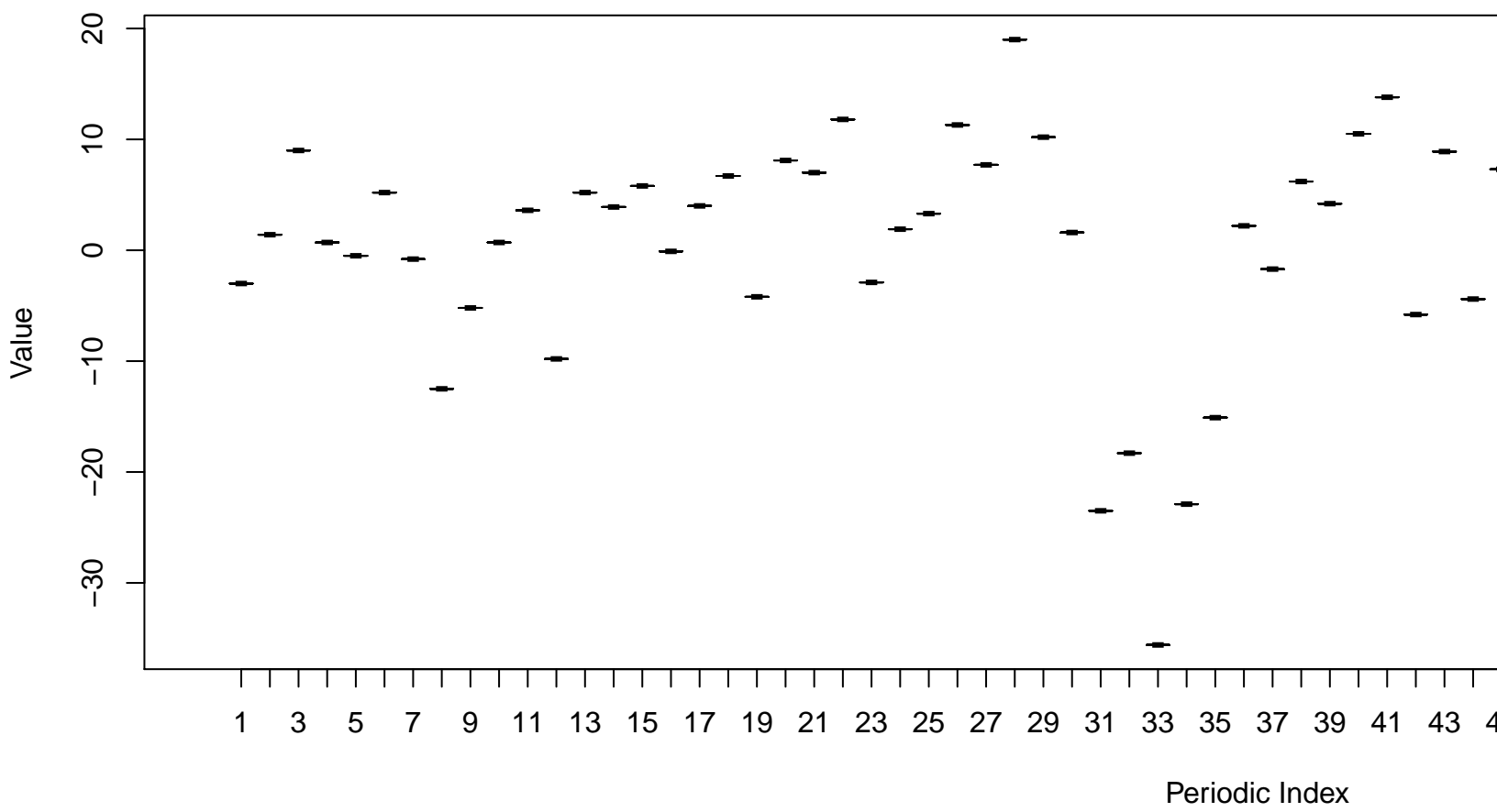
Notched Box Plots – Differenced Periodic
