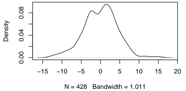
Kernel Density Plot of Residuals
