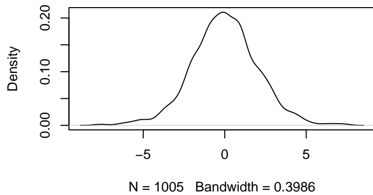
Kernel Density Plot of Residuals
