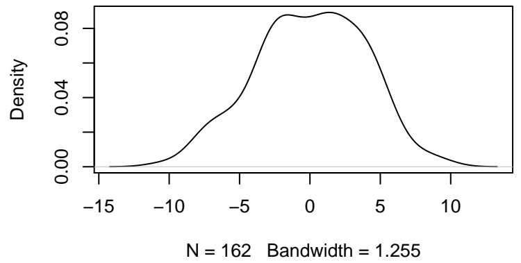
Kernel Density Plot of Residuals
