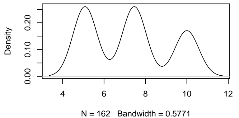
Kernel Density Plot of Predictions
