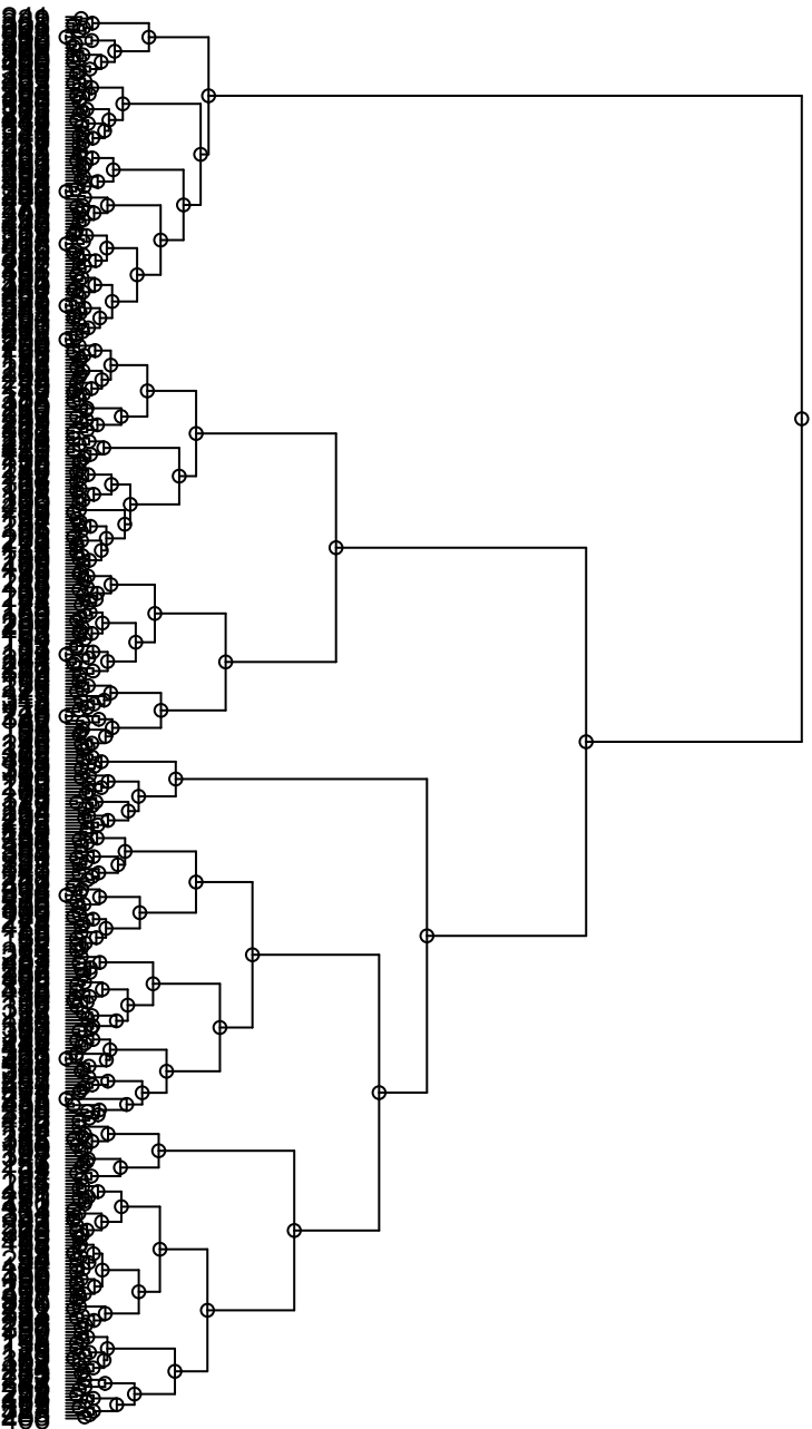
Dendrogram
